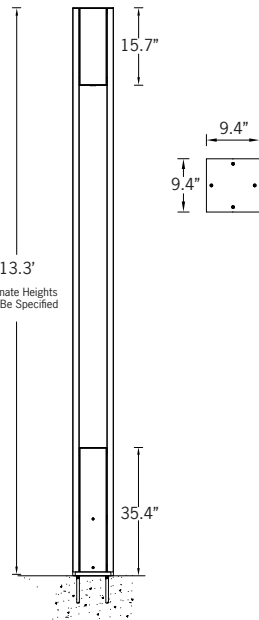
Mounting Detail
