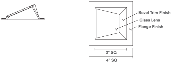
Trimmed - B3SWF-FC1
