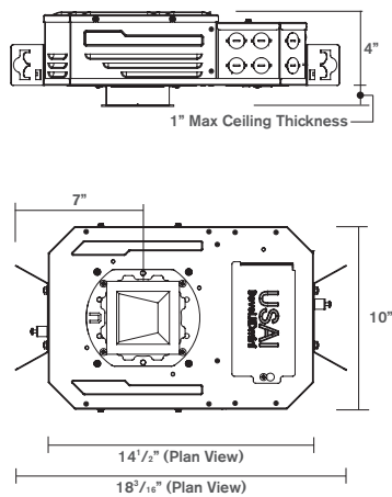
Flat Adjustable Housing - FTA
