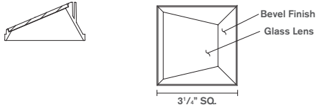
Trimless - B3SWL-FC1
