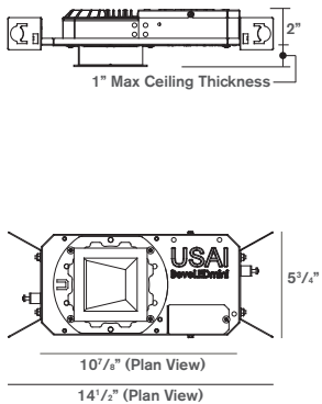
Flat Housing - FT
