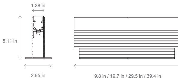
Ground Liner® High recessed box+luminaire.
