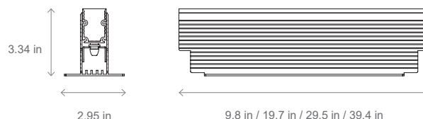
Ground Liner® Low recessed box+luminaire.
