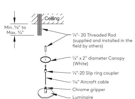
PL9LR Cable (C) Suspension Detail (Non-Feed location(s) only)
