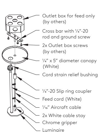
PL9LR Cable (C) Suspension Detail (Feed location(s) only)
