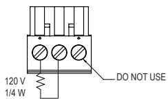
3 POSITION FEMALE CONNECTOR WITH TERMINATION CONNECTOR.
