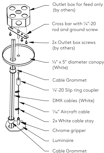
PL9LR Cable (C) Suspension Detail (DMX Feed location(s) only)
