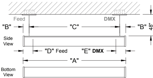
Cable (C) Mounting - Dimensions
