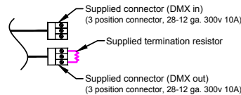
DMX connector detail
