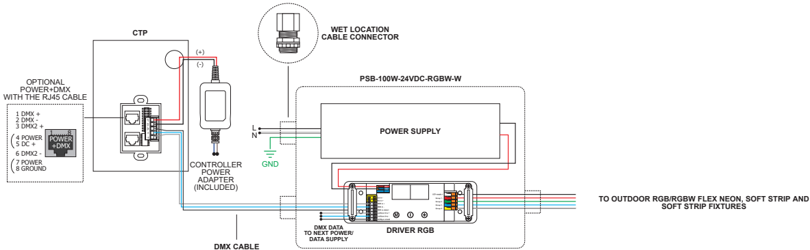
WIRING DIAGRAM FOR OUTDOOR RGB/RGBW FLEX NEON, SOFT STRIP, AND SOFT STRIP FIXTURES
