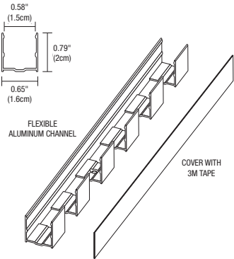
FLEXIBLE ALUMINUM CHANNEL
