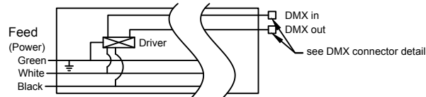
Dimming - DMX eldoLED POWERdrive (DMX) (Individual fixtures)
