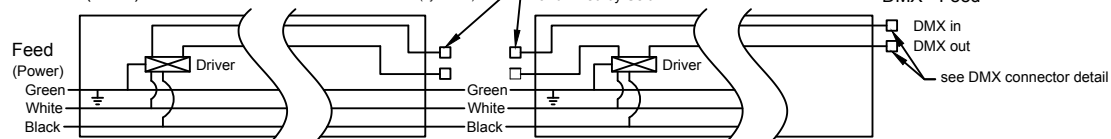
Dimming - DMX eldoLED POWERdrive (DMX) (Runs)
