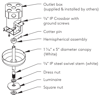
L1DI Swivel Stem (S) Suspension Detail (feed wires through stem supplied by others)
