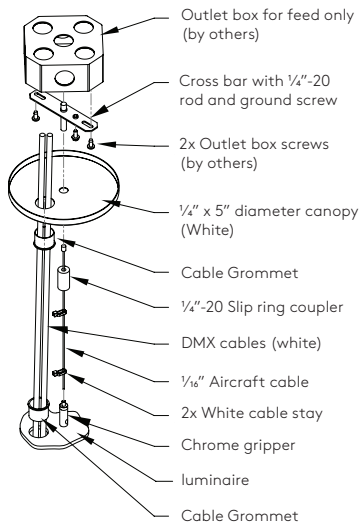
L10 Cable (C) Suspension Detail (DMX Feed location(s) only)
