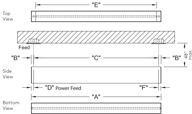
Swivel (S) & Rigid Stem (RS) Mountings - Dimensions
