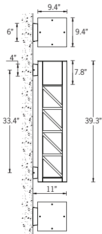
Mounting Detail
