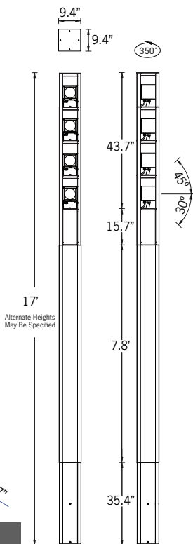
Mounting Detail
