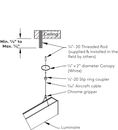
PXLDI Cable (C) Suspension Detail (Non-Feed location(s) only)
