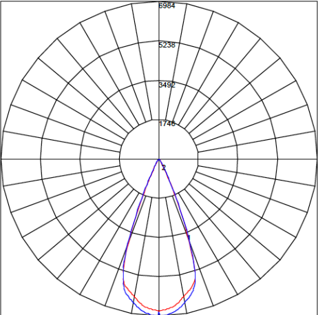
Maximum Candela = 6984.45 Located At Horizontal Angle = 0, Vertical Angle = 5 # 1 - Vertical Plane Through Horizontal Angles (190 - 270) # 2 - Vertical Plane Through Horizontal Angles (0 - 180)
