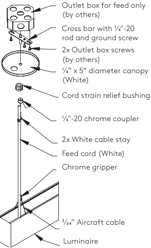
PXLDI Cable(C) Suspension Detail (Feed location(s) only)
