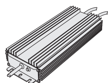
APS-300-24-IP Powers 2 x 50 Unit Run 300W, 24VDC, IP66 Wet location, 100-277VAC Input
