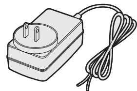
APS-30-24 Powers 1 x 8 Unit Run 30W, 24VDC, Dry location, Wall Plug 100-240VAC (47-63Hz) Input
