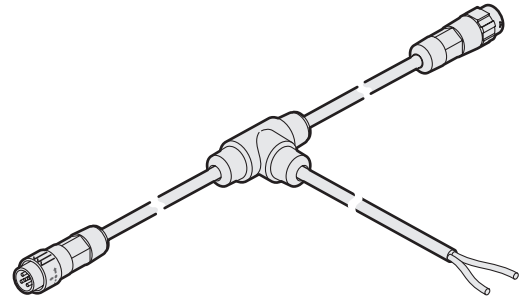
ADOT1-V2 1' "T" Link Cable For AL Dot (extends DMX link while injecting a new 24VDC line)
